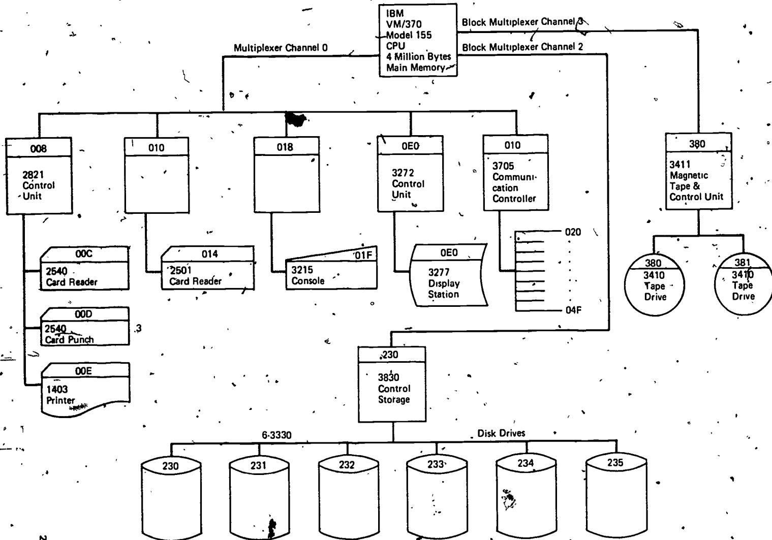
Figure 3 - JSUCC VM/370 System Configuration
